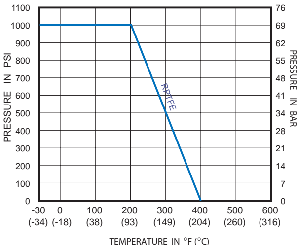
Pressure Vs. Temperature Chart
